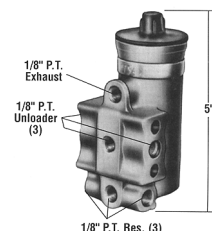
D-2 Governor
