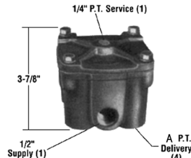
R-12 Relay Valve with
