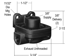
QR-1 Quick Release Valve
