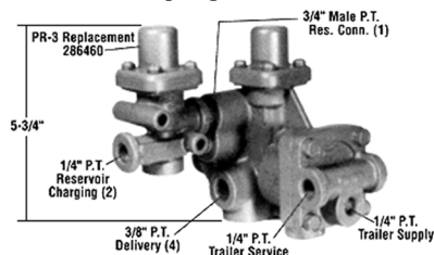
SR-4 Spring Brake Valve
