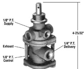
PP-7 Trailer Supply Valve
