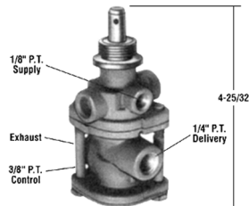
PP-7 Trailer Supply Valve
