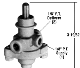
PP-1 Control Valve
