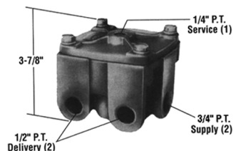
R-12 Relay Valve
