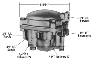
RE-6 Relay Emergency Valve
