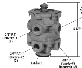
Dual Brake Valve
