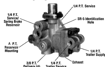
SR-5 Anti-Compounding Spring Brake Valve
